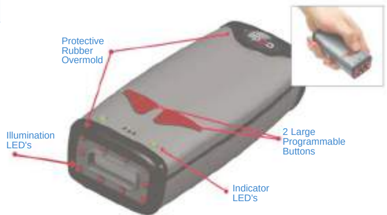
Code Reader 2.0 in Hand Format
